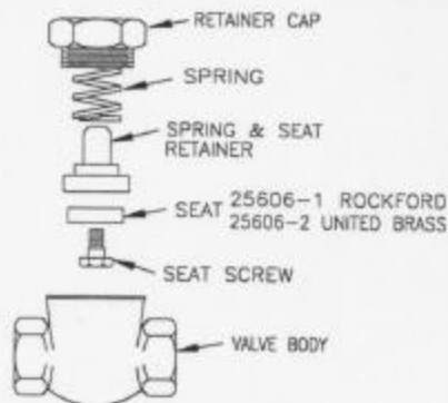
QUICK EXHAUST VALVE 17799
