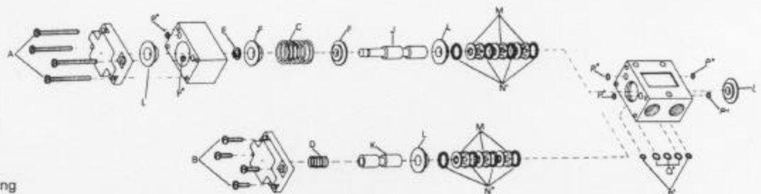
30632 - PUSH BUTTON SPOOL VALVE 30633 - PILOT OPERATED SPOOL VALVE 30860-3 KIT FOR SPOOL VALVES
