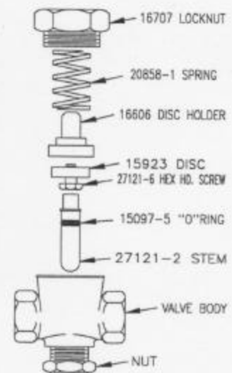
1/4" AIR WHISTLE VALVE WEAKER SPRING 20858
