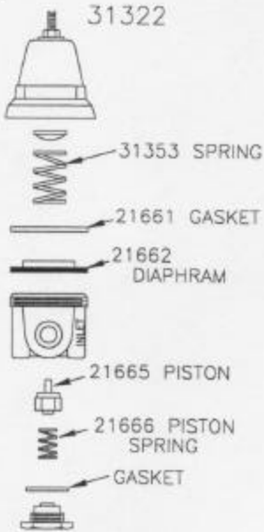
1/4" VARIABLE REGULATOR 31322
