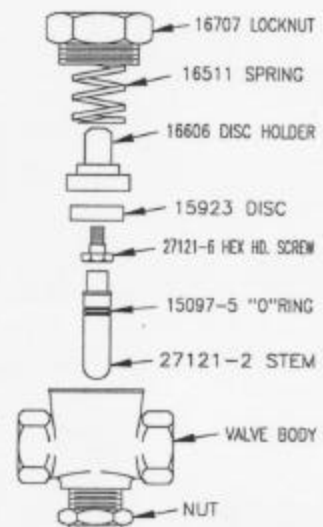
1/4" AIR WHISTLE VALVE 15100
